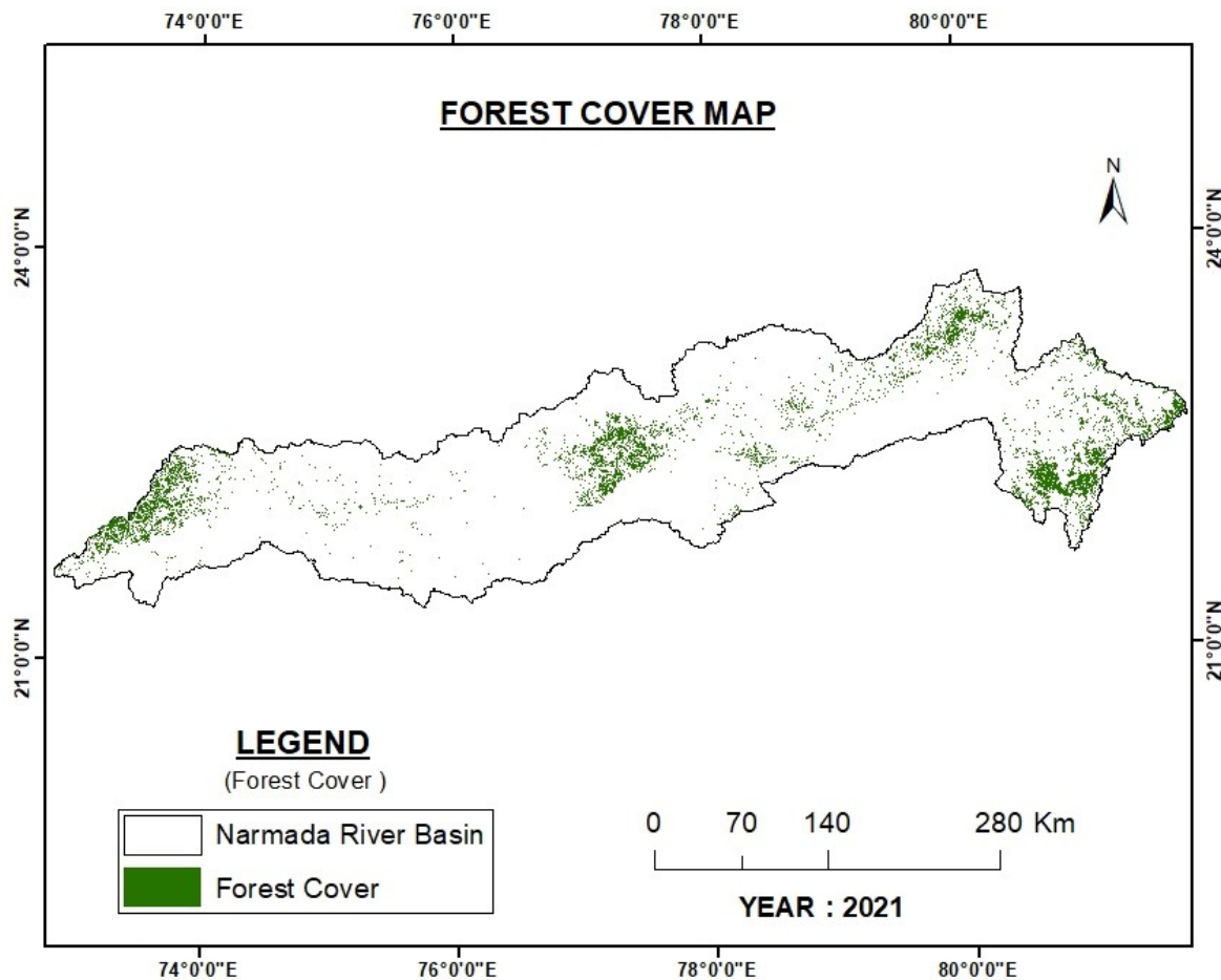
Figure 4: Forest cover area of the year 2021
