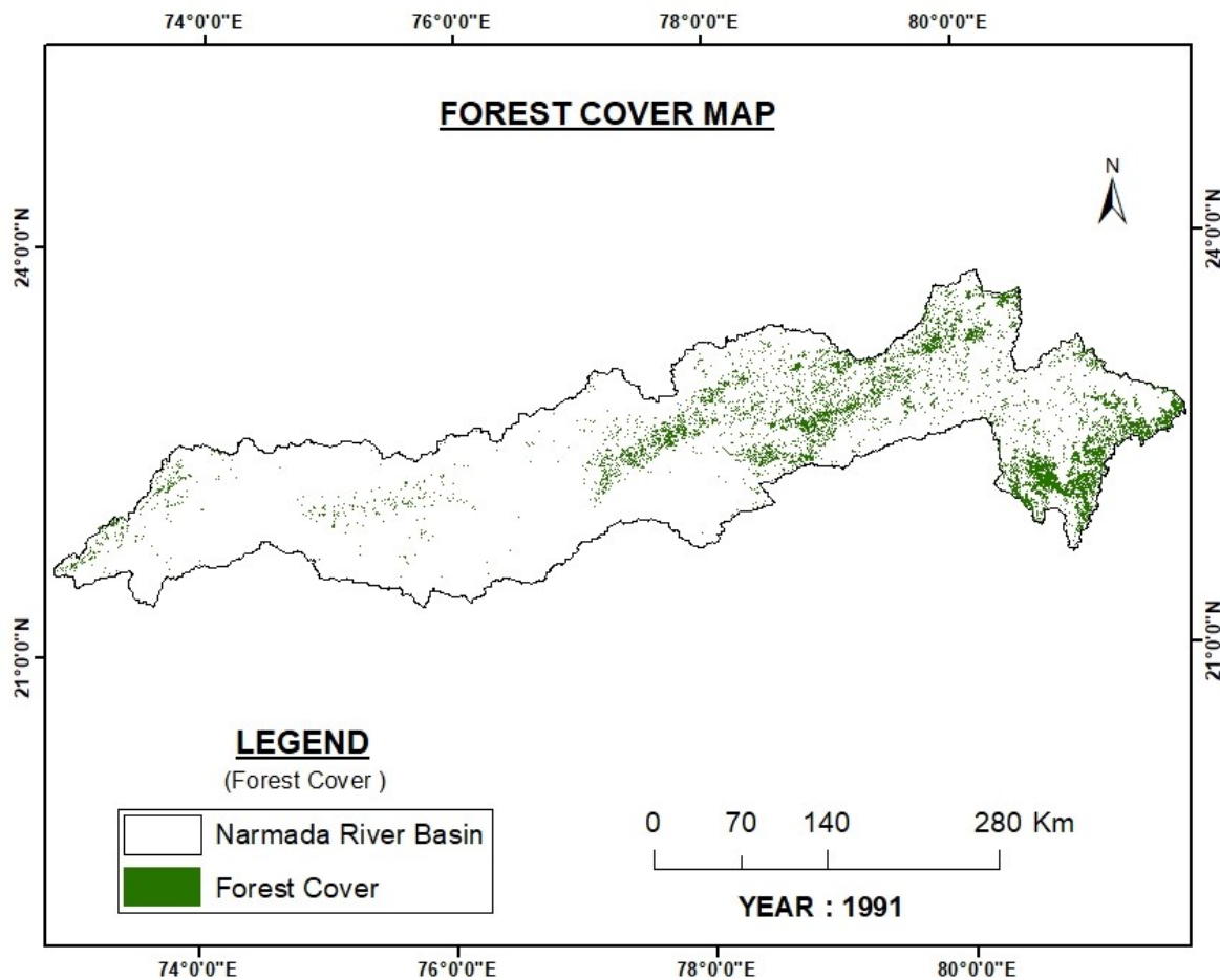
Figure 3: Forest cover area of the year 1991
