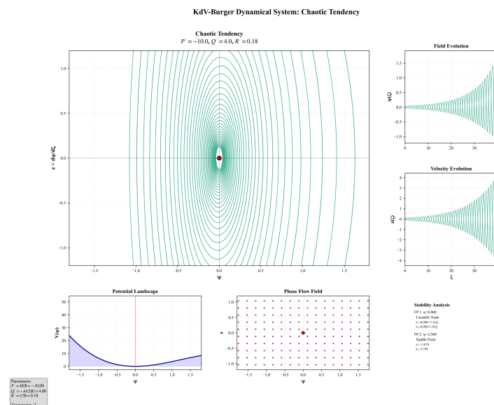
Figure 1: Chaotic waveform evolution under moderate nonlinearity and dissipation, showing intermittent irregularity and waveform distortion.
