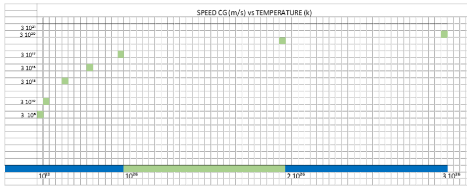
Figure 7: Represents the variation of speed C_G , as a function of temperature T , inside a black hole.
